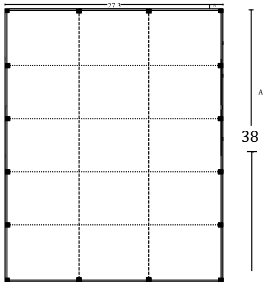
FLOOR PLAN
